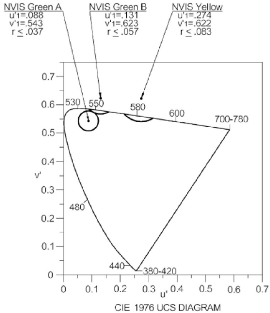
FIGURE 7. Color limits for NVIS night vision goggle compatible colors.
