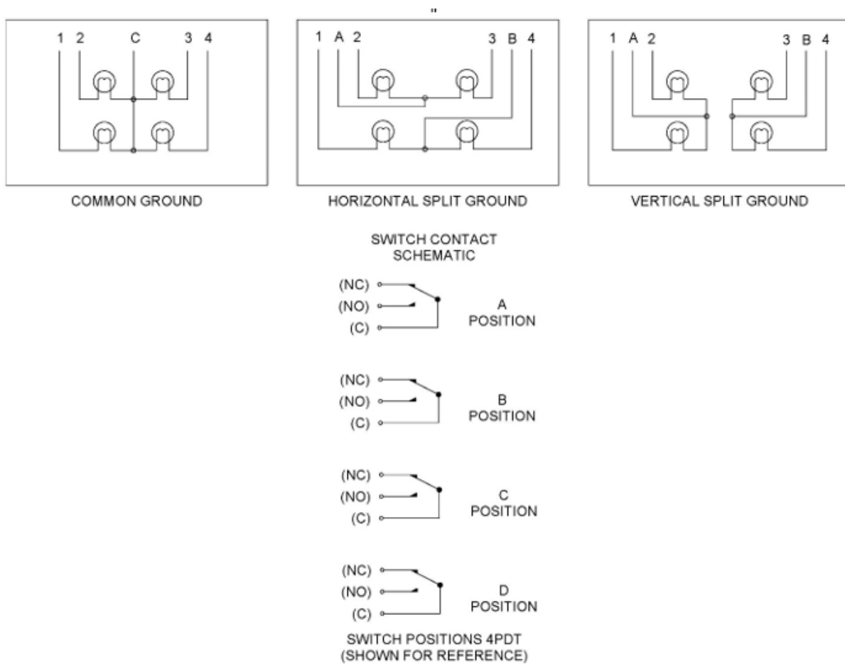
FIGURE 4. Switch and lamp circuit schematics and termination arrangements and identification.
