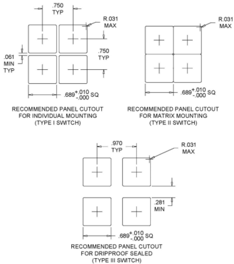
FIGURE 6. Recommended panel cutouts.
