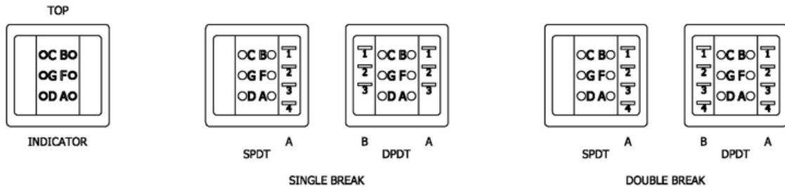
FIGURE 12. Switch poles and lighting circuit terminal arrangements and identification.
