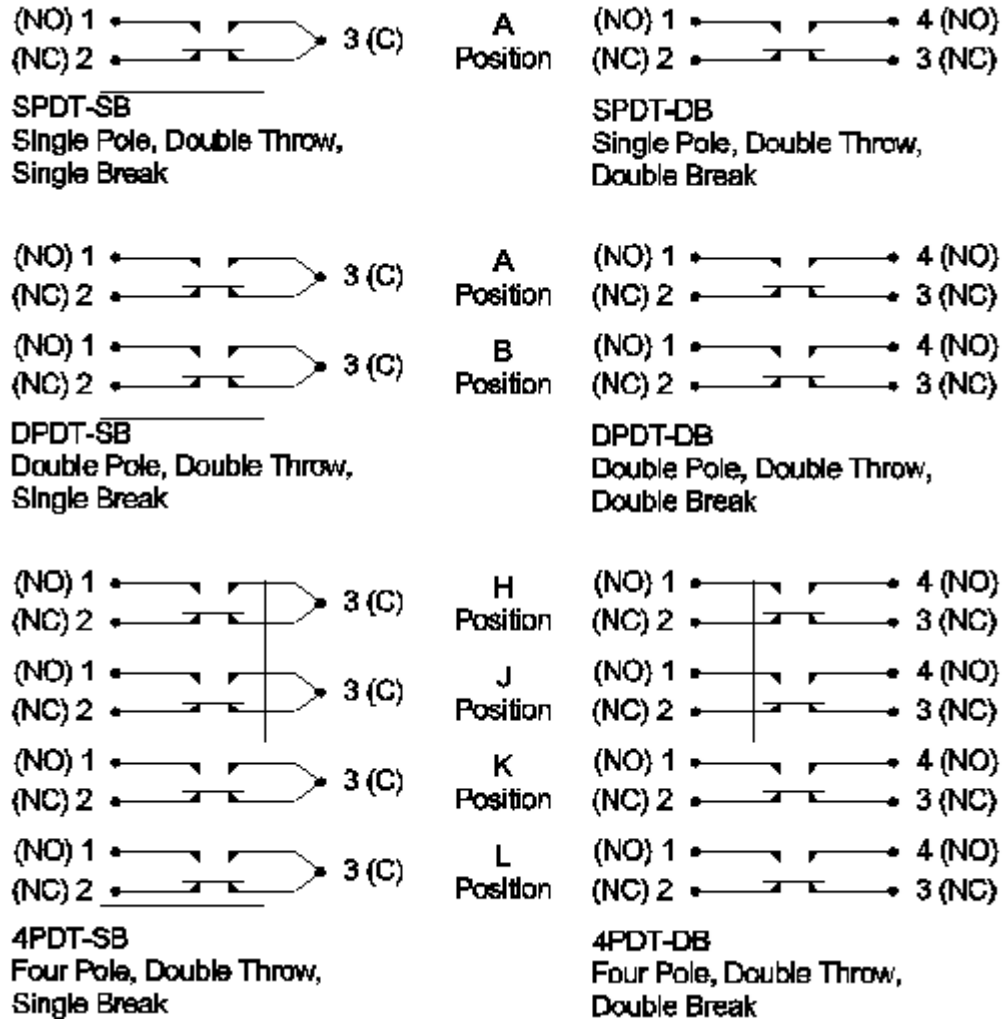
FIGURE 9. Switch circuit configurations, schematics.
