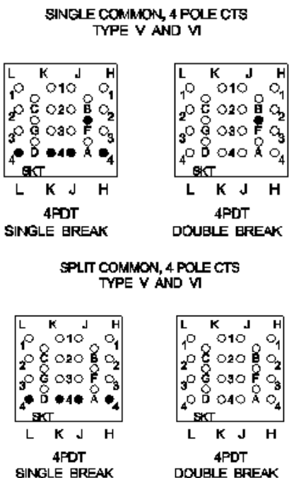
FIGURE 12. Switch poles and lighting circuit terminal arrangements and identification - Continued.
