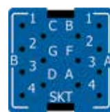
18-442 NEXSYS Connector Plug* (For Compact VIVISUN bodies with NEXSYS components)
